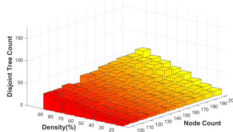
Fig. 5: Number of the disjoint trees found by the traditional DFS against the network density and number of nodes.
