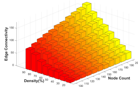
Fig. 4: Edge connectivity of the networks against the network density and number of nodes.
